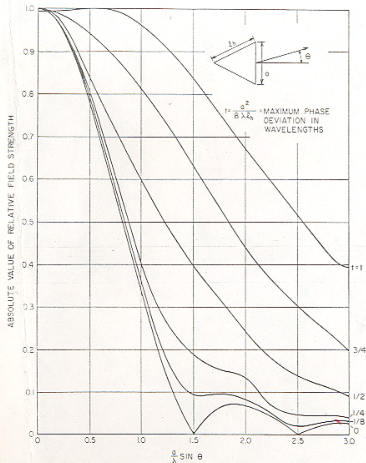
FIG. 15-5 Universal radiation patterns of horns flared in the H plane (sectoral or pyramidal).
